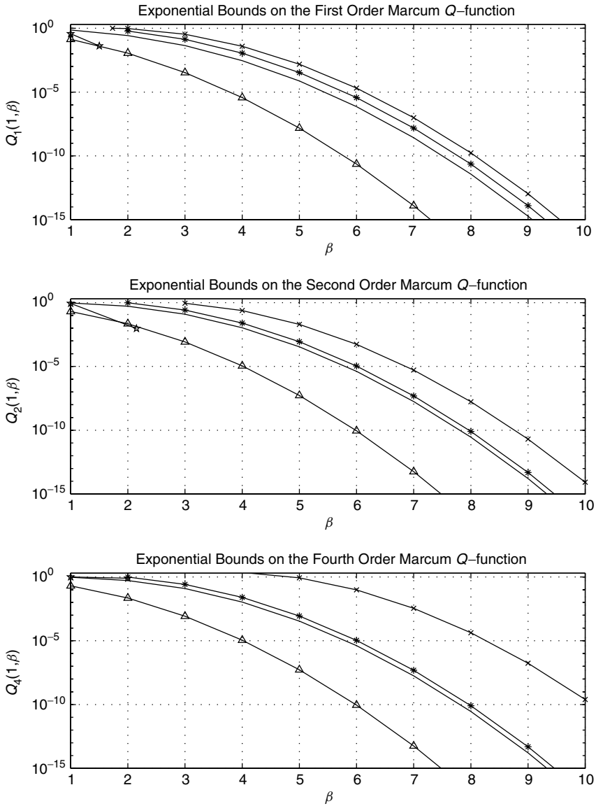
Figure 4.2. Plots of Q_1(1, \beta) , Q_2(1, \beta) , Q_4(1, \beta) , and their bounds versus \beta : —, Exact; *, upper bound (4.57a); \times , Chernoff upper bound from Ref. 23; \star , Chernoff lower bound from Ref. 23; \Delta , lower bound of (4.62).
