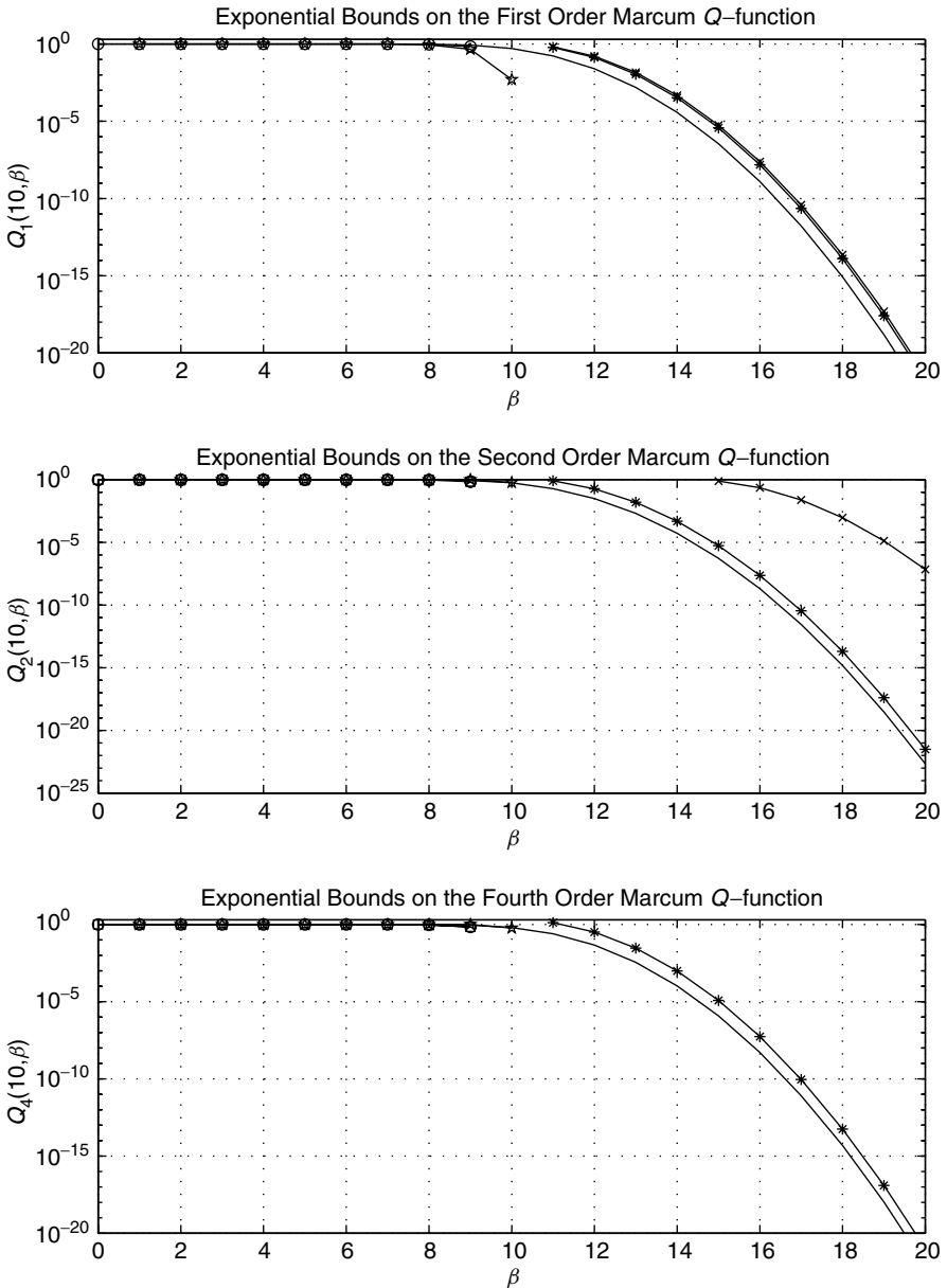
Figure 4.4. Plots of Q_1(10, \beta) , Q_2(10, \beta) , Q_4(10, \beta) , and their bounds versus \beta . —, Exact; *, upper bound of (4.57a); ×, Chernoff upper bound from Ref. 23; ☆, Chernoff lower bound from Ref. 23; △ lower bound of (4.62). Note that the lower bound given by (4.62) and the Chernoff upper bound from Ref. 23 ( m = 4 ) are out of the range of the plot.
