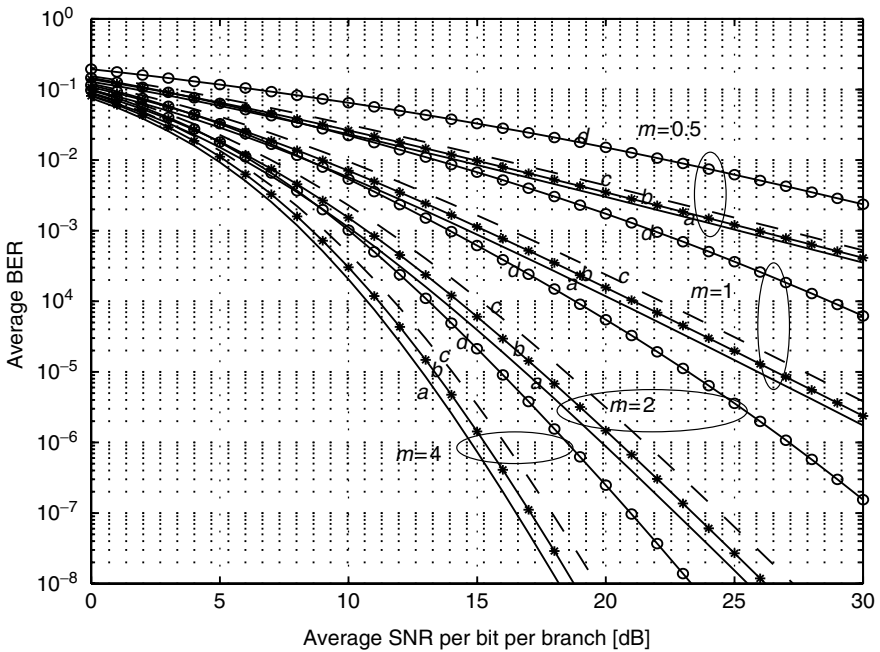
Figure 9.41. Average BER of BPSK with SSC versus average SNR per branch \bar{\gamma} for various values of the correlation coefficient [ \rho = (a) 0, (b) 0.3, (c) 0.6, and (d) 0.9 ] over Nakagami- m fading.
