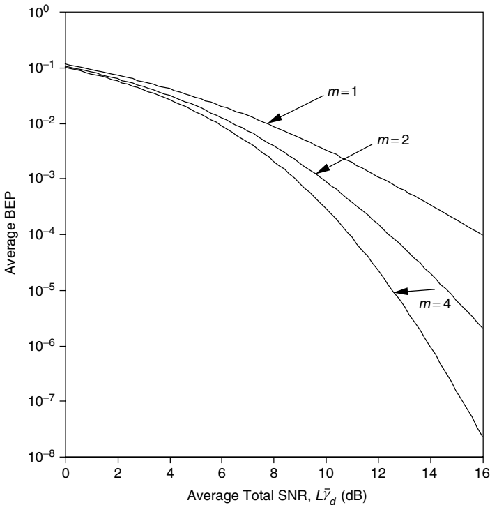
Figure 10.7. Average BEP of the optimum combiner in Nakagami- m fading with a single fading co-channel interferer; \bar{\gamma}_d = \bar{\gamma}_l , L = 4 .
